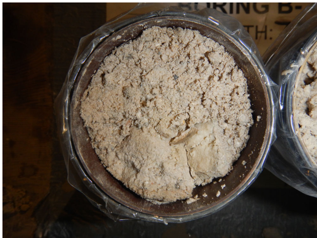
Boring B-13, Sample 5, Depth: 7.0' - 8.5'
