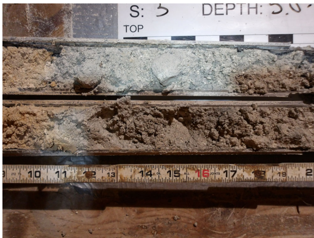
Boring B-21, Sample 3, Depth: 5.0' - 7.0'
