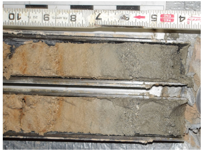
Boring B-2, Sample 5, Depth: 5.5' - 7.0'
