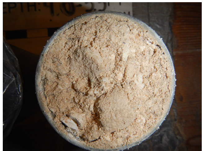
Boring B-10, Sample 3, Depth: 4.0' - 5.5'
