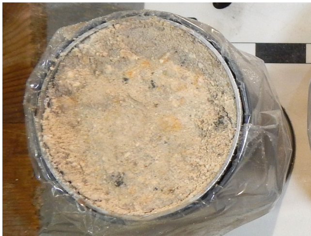
Boring B-15, Sample 3, Depth: 4.0' - 5.5'
