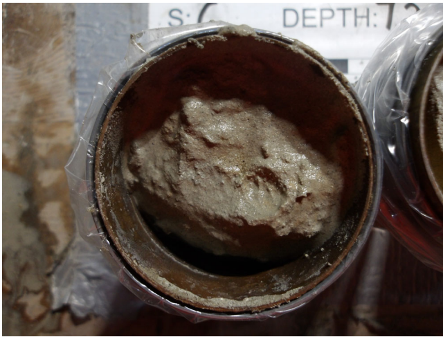
Boring B-4, Sample 6, Depth: 7.3' - 8.8'
