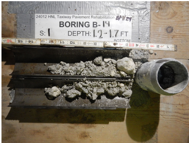
Boring B-14, Sample 1, Depth: 1.2' - 1.7'
