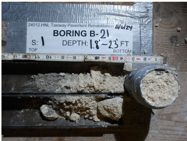
Boring B-21, Sample 1, Depth: 1.8' - 2.3'
