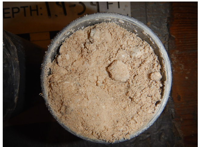
Boring B-10, Sample 2, Depth: 1.9' - 3.4'
