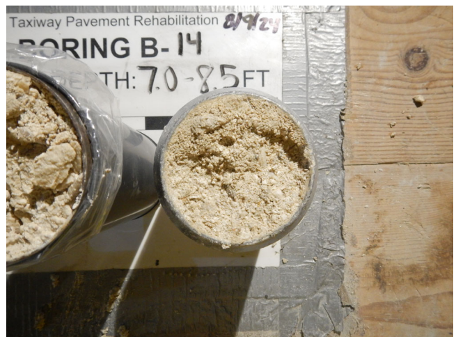
Boring B-14, Sample 5, Depth: 7.0' - 8.5'
