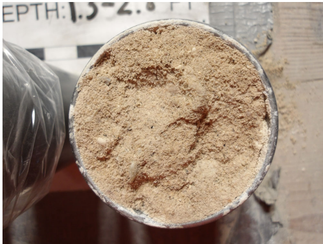
Boring B-6, Sample 2, Depth: 1.3' - 2.8'
