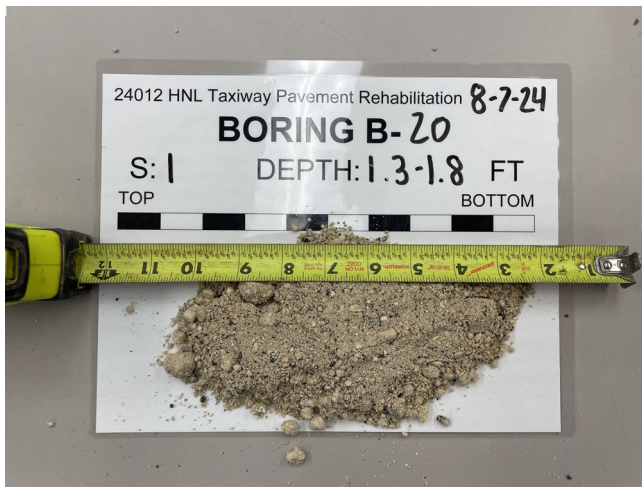
Boring B-20, Sample 1, Depth: 1.3' - 1.8'
