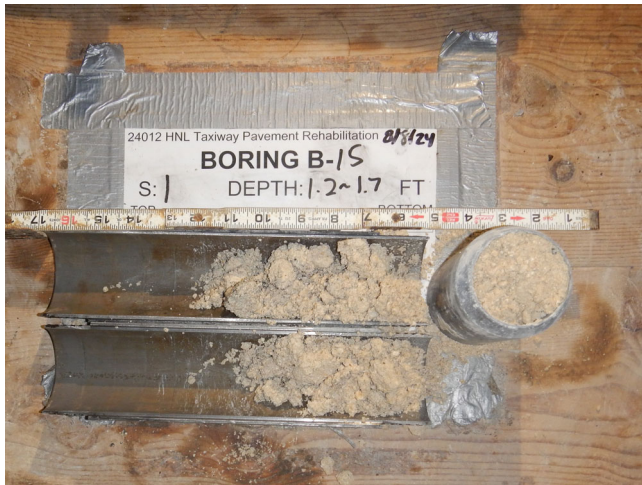
Boring B-15, Sample 1, Depth: 1.2' - 1.7'
