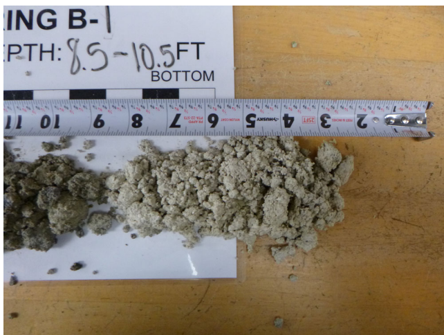
Boring B-1, Sample 7, Depth: 8.5' - 10.5'
